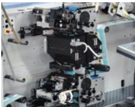
UV Flexo/Siebdruck
